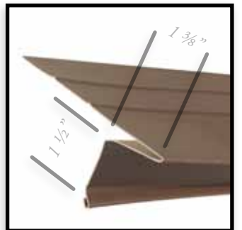
Drip Edge 1 3/8" drip projection Available in Copper, 13 Aluminum Colors & Galvalume
