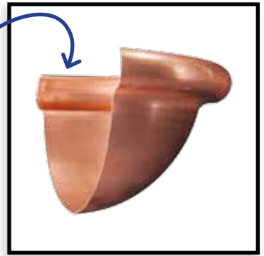
Reverse Bead Spherical End Cap, installs left or right, available in 5", 6" & 8" in Copper & Chromated Aluminum
