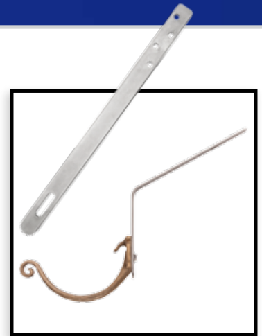
Roof Bar, Copper & Stainless Steel, 1" wide x 3/16" thick, with 1 1/2" slot to adjust pitch. Used with Cast Fascia Brackets & Bar Brackets
